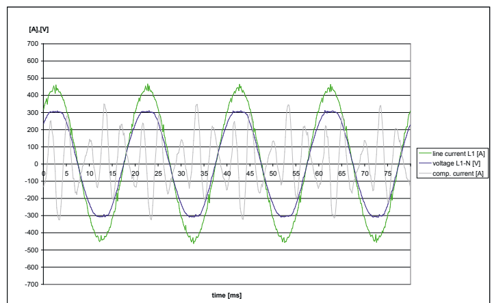
Voltage and input current with ECOsine™ Active as well as the compensation current of the filter
